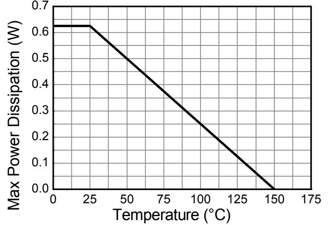
Derating Curve
